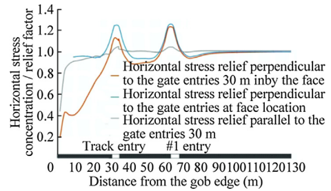
Fig. 14. Horizontal stress concentration and relief factors over the chain pillars.
