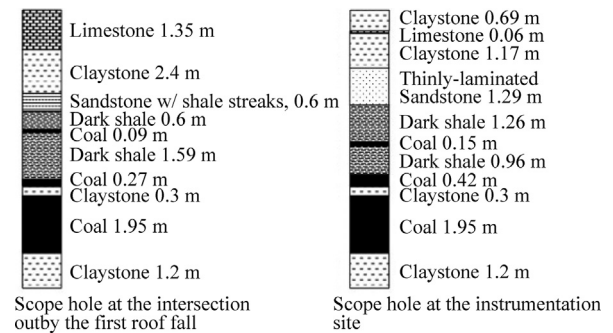
Fig. 2. Geologic columns drawn with the scoping results.
