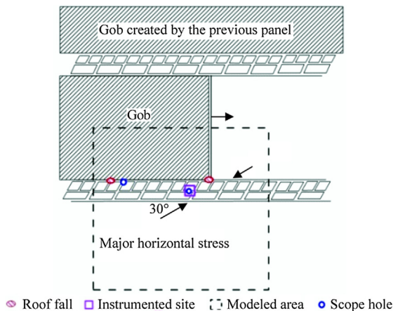
Fig. 1. Panel layout and the instrumentation site.
