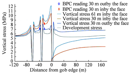
Fig. 8. Vertical stress across the gate entries.
