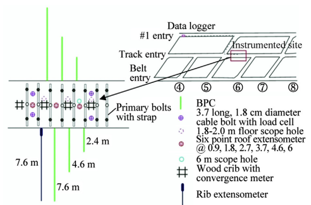
Fig. 3. Instrumentation layout in the track entry.
