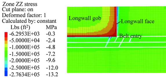
Fig. 7. Vertical stress distribution over the headgate area.
