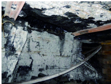
Fig. 12. Cutter developed at the inby corner of the intersection.
