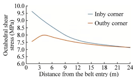
Fig. 13. Octahedral shear stress along the length of the crosscut 1 m above the roofline when the face is 15 m from the intersection.
