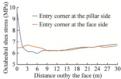
Fig. 16. Octahedral shear stress at the belt entry corner 1 m above the roofline in a left-handed panel.
